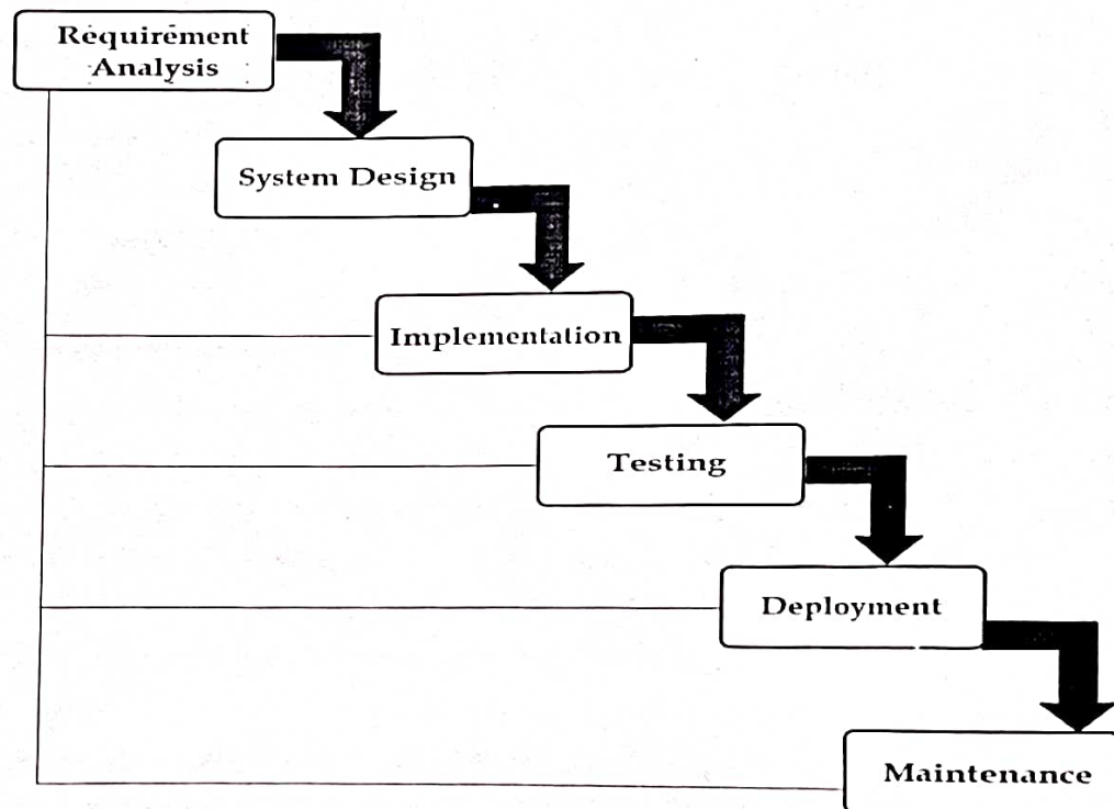
Fig. 3.11 Waterfall model
