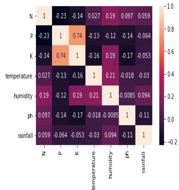
Fig. 5 Data Analysis as Heatmap
