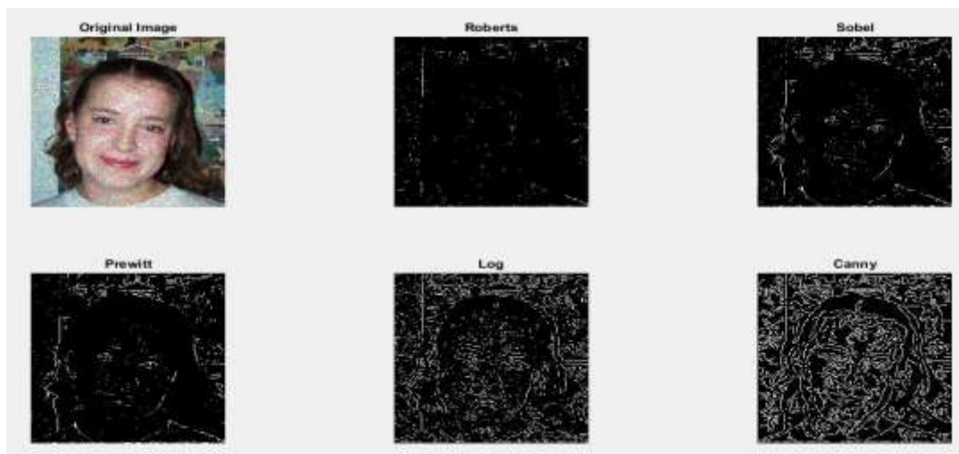
Figure 11. Salt & Pepper Noise Effect on Face Image with the Outcome of Different Edge Detection Techniques
